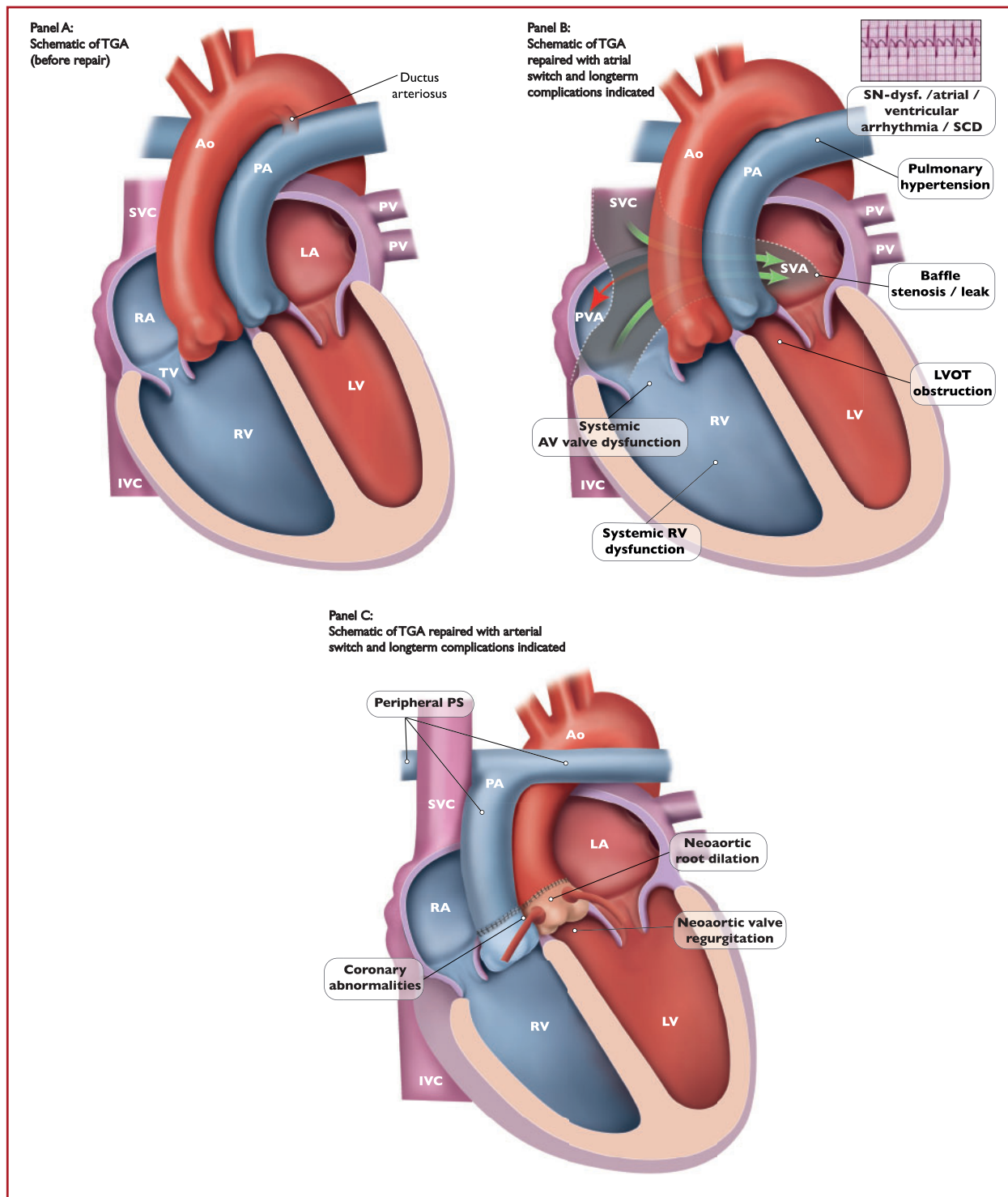
Figure 9 Management of transposition of the great arteries: long-term complications to address during follow-up. Ao = aorta; AV = atrioventricular; IVC = inferior caval vein; LA = left atrium; LV = left ventricle; LVOT = left ventricular (subpulmonary) outflow tract; PS = pulmonary stenosis (supravalvular/pulmonary artery branch); PV = pulmonary vein; PVA = pulmonary venous atrium; RA = right atrium; RV = right ventricle; SCD = sudden cardiac death; SN-dysf. = sinus node dysfunction; SVA = systemic venous atrium; SVC = superior vena cava; TV = tricuspid valve.
